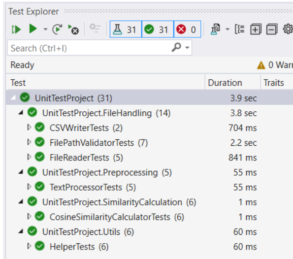
Fig 17: Unit Tests
